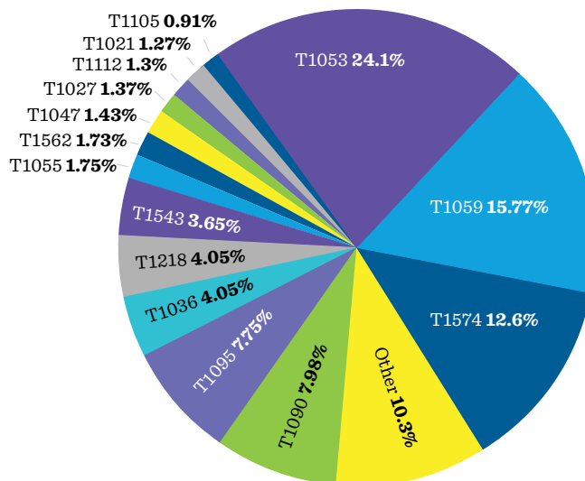
Figure 1 Total Dataset Technique Breakdown
