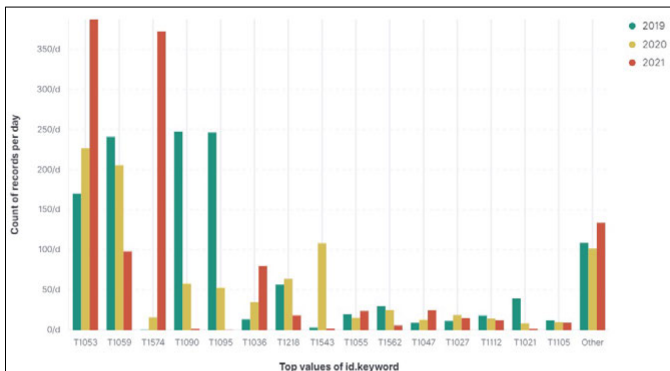
Figure 11 Most Observed Techniques Count Per Day 2019-2021
