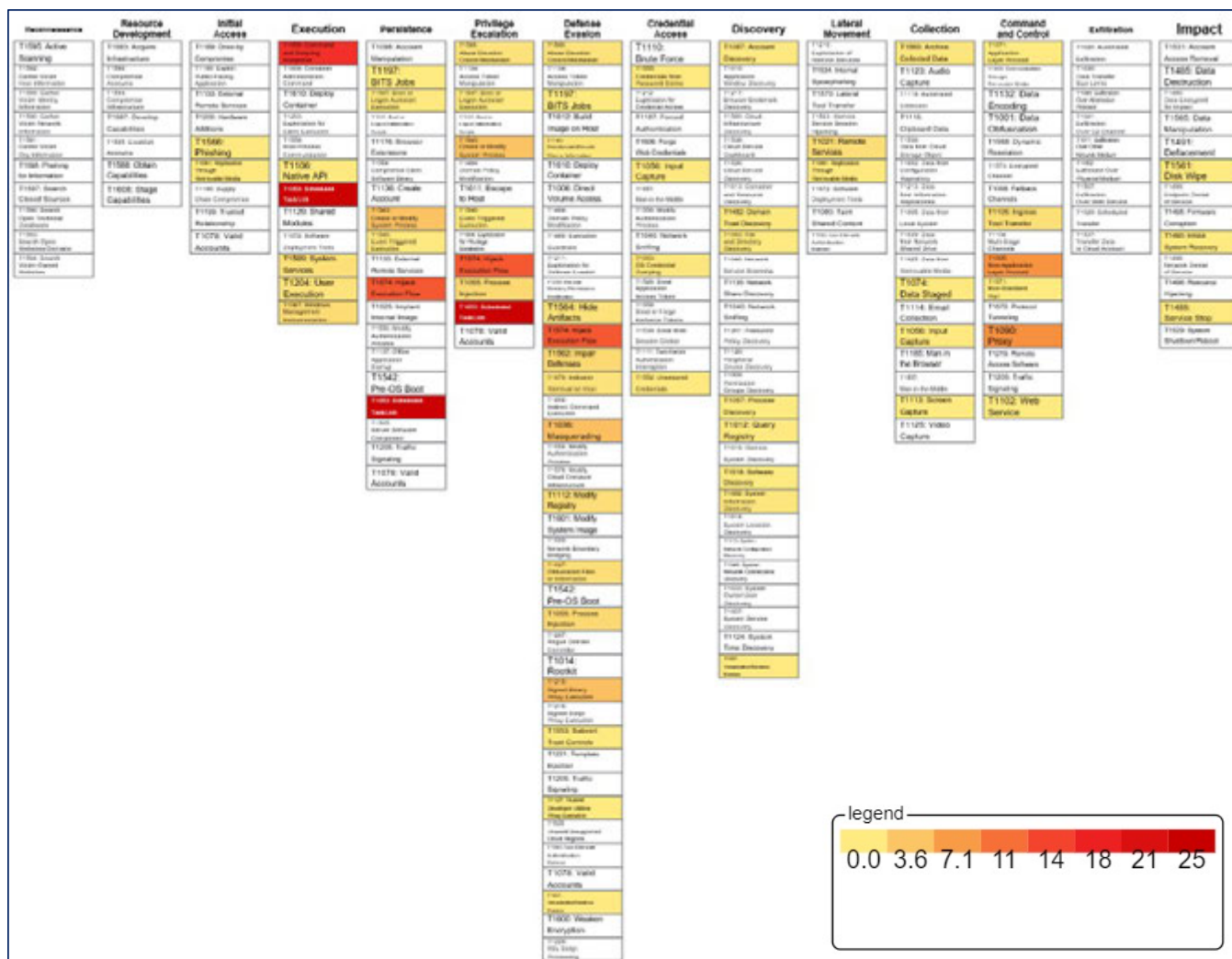
Figure 14 Heatmap of the 50 Most Observed Techniques Scored by the Percentage of the Total Dataset Represented
