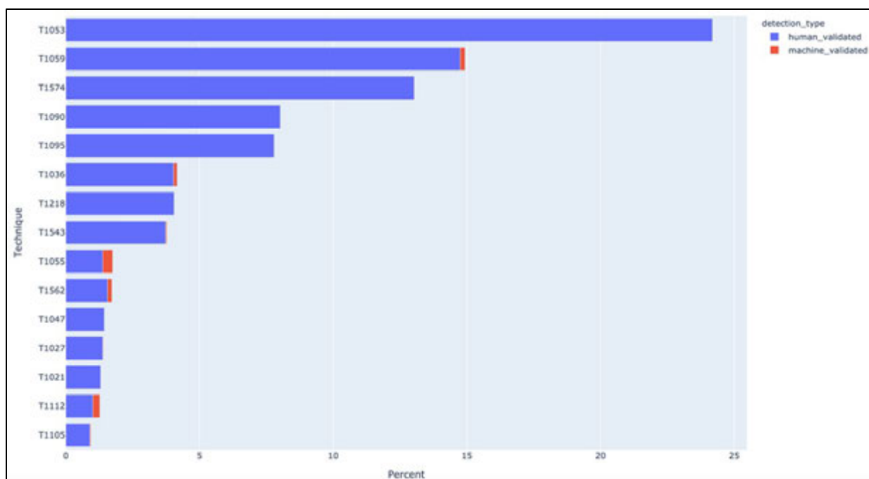
Figure 17 Most Observed Techniques Detection Type Breakdown
